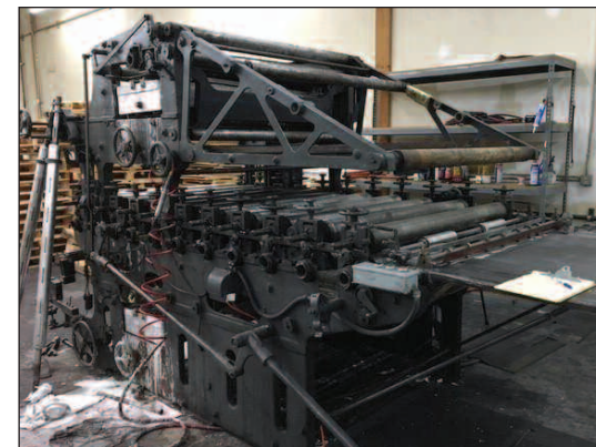
Samuel Parry Machine Co. Savage Universal 00 Glue Press
