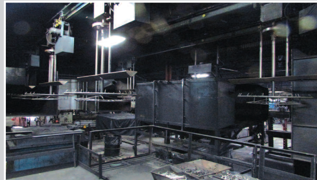
RCK Industries Shot Peening Line with Bronco 2-Wheel Shot Peener
