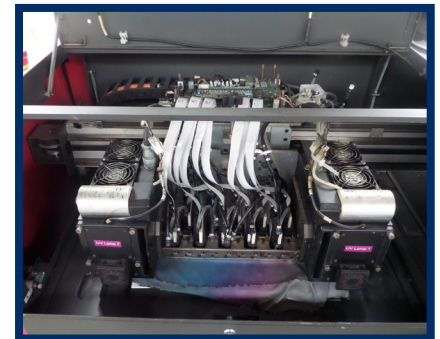
View of Print Heads
