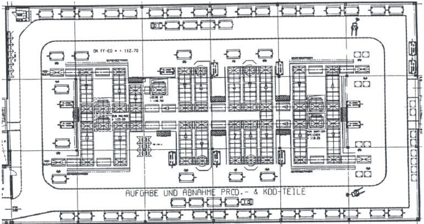
3 rd Level: Loading and Unloading of Parts (this floor space is not necessarily required completely)
