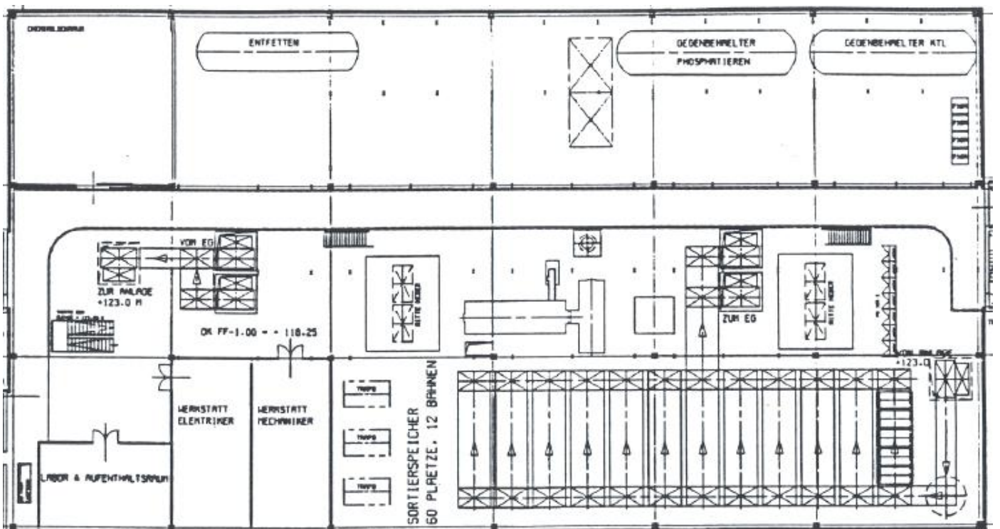
4 th Level: Degreasing and Washing
