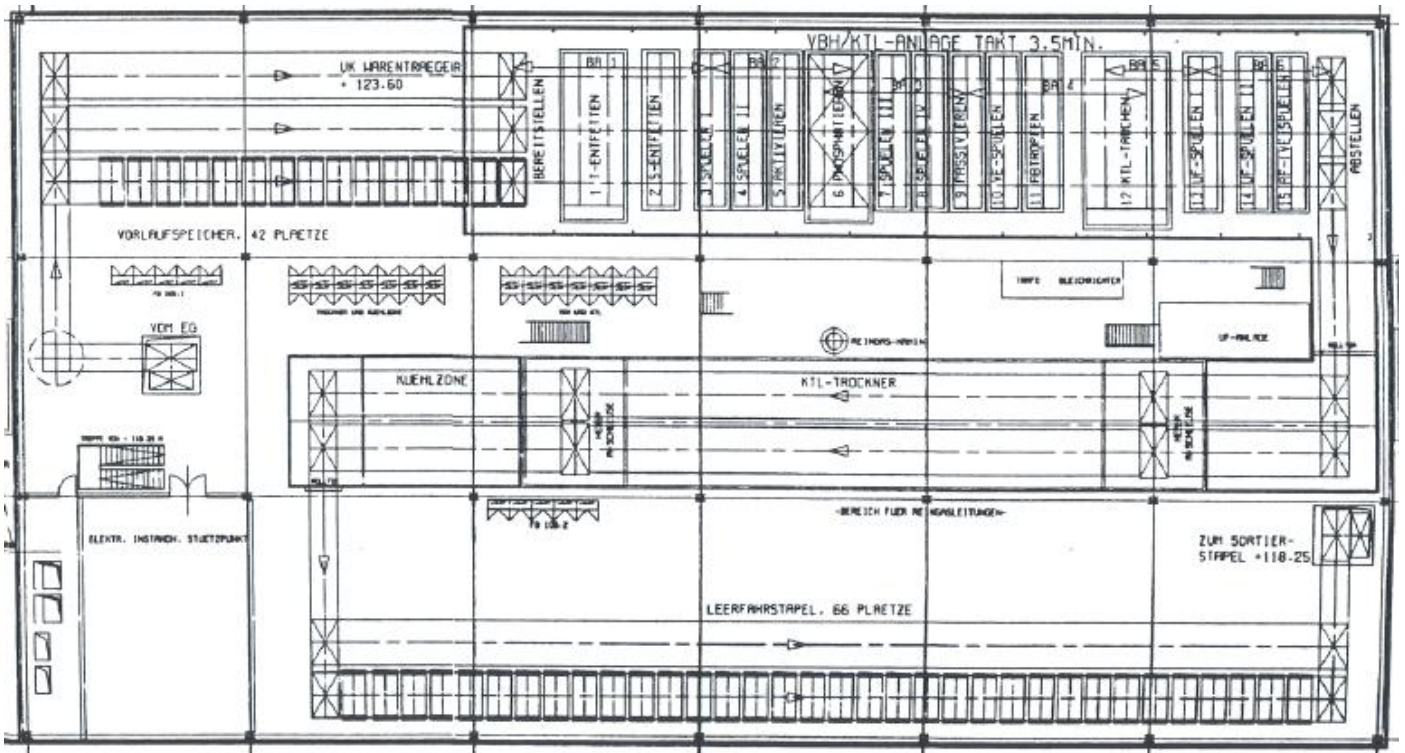
5 th Level: Immersion Painting Line and Drying/Coolant Line
