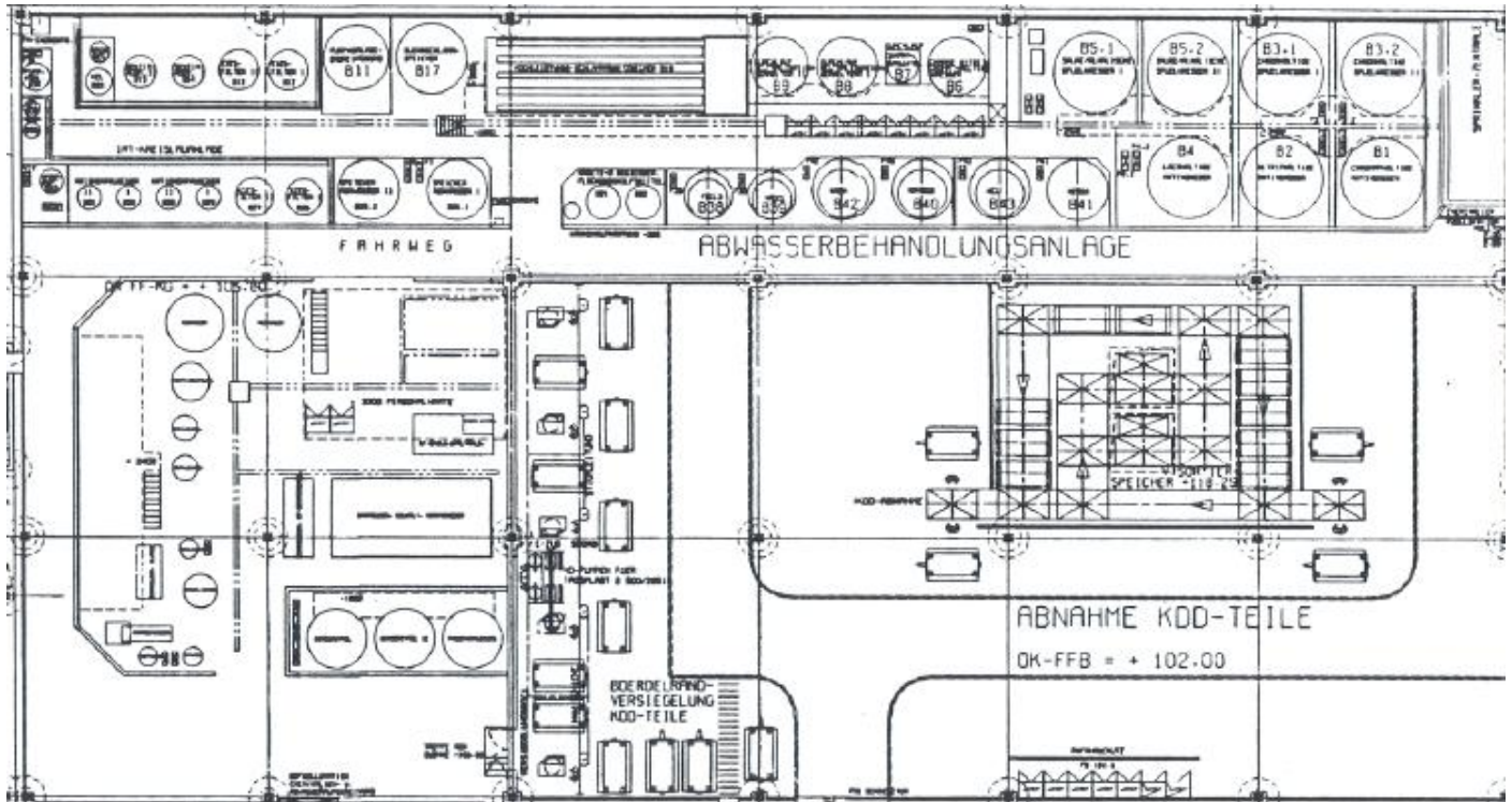
Ground Level: fluid Media Treatment
